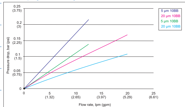
Pressure drop diagram for 10", 20" Big Blue®
