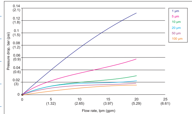
Pressure drop diagram for 10", 20" Big Blue®
