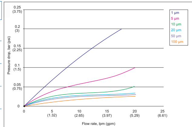
Pressure drop diagram for 20" cartridges
